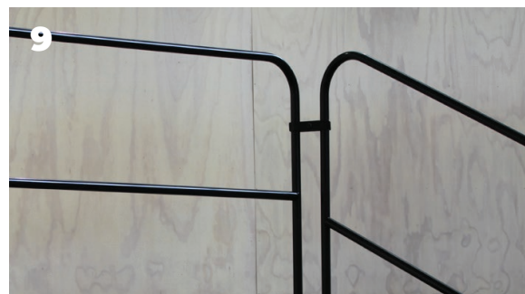
Secure Hand Rails with a Hand Rail Clamp.
