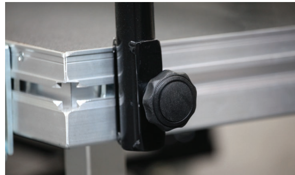
Hand Rail T-Bolt and Hand Wheel
