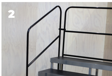
Add Back and Side Safety Rails. Secure with Rail Clamps.
